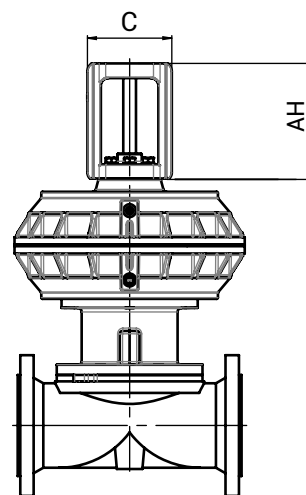
Control function 2 + 3 Mounting type with NAMUR mounting bracket (code NH0)
