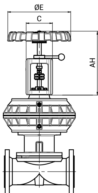
Control function 2 Mounting type with NAMUR mounting bracket and handwheel (code NH)
