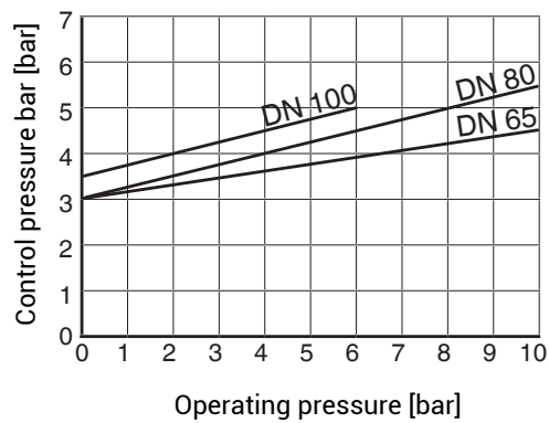
Actuator 3/F, 3AF, 3/D, 3AD
